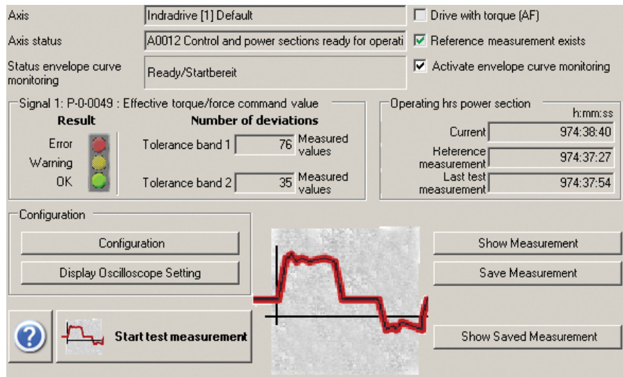
When Envelope Curve Monitoring is loaded to an axis using Rexroth’s IndraWorks software, the user interface simplifies the process to visualize and configure the two defined tolerance bands.
