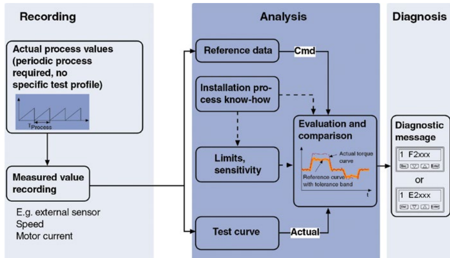
Envelope Curve Monitoring allows you to analyze and diagnose a variety of configurable signal measurements based on tolerance levels defined by the user.
