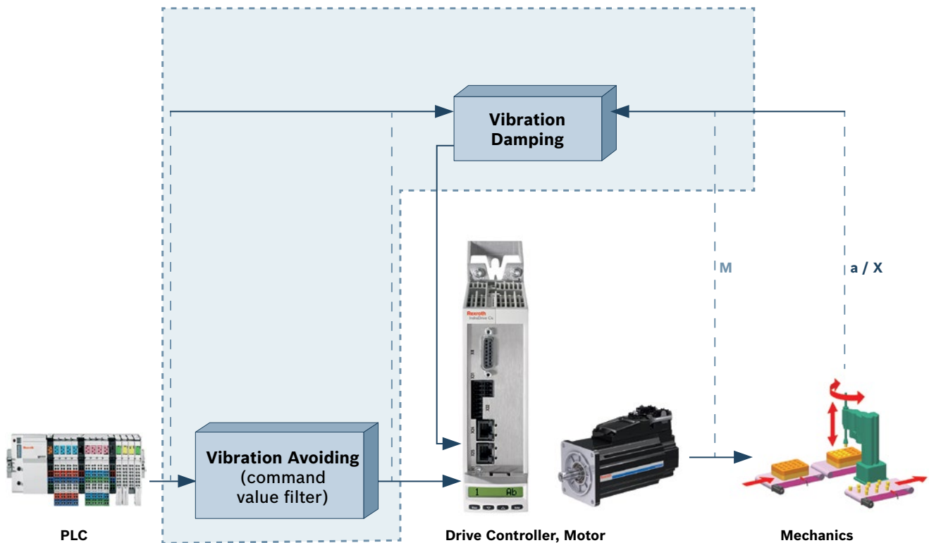
A Rexroth drive system with Adaptive System technology can implement vibration damping and avoiding together with or without a PLC.
